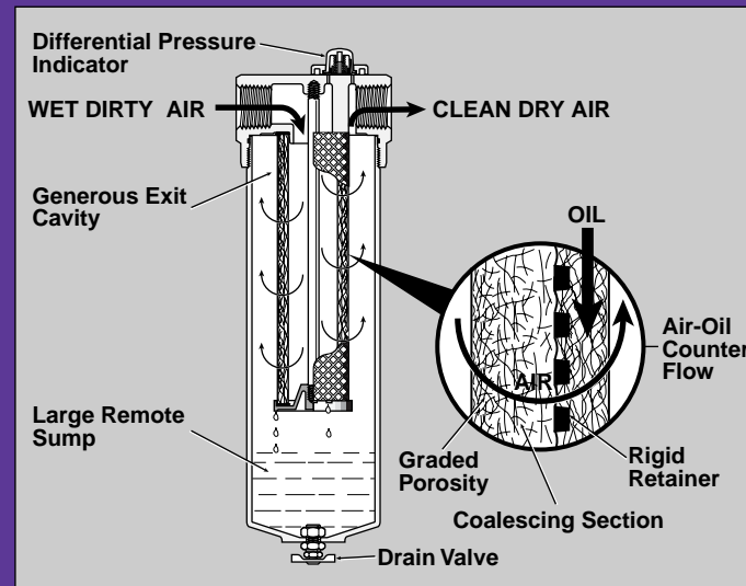
This coalescing filter depicts how the air flows from the inside out. This housing contains a coalescer with a built in prefilter.
