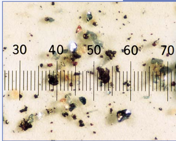
Actual pictomicrograph of particulate contaminants (Magnified 100x Scale: 1 division = 20 microns)
